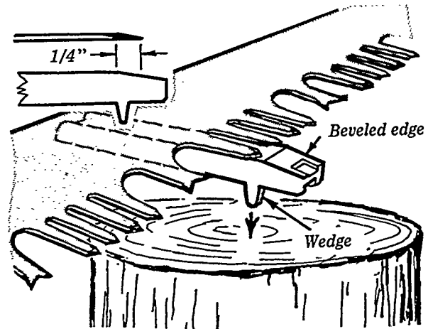
Using a setting stake on a stump.
