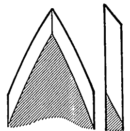
Cutter tooth shape for hardwood.
