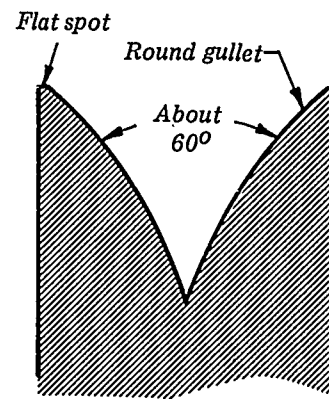
Shaping a raker tooth (straight raker).
