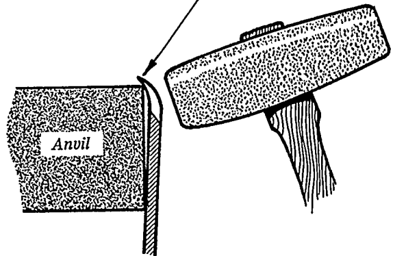
Correcting an "over-set" cutter tooth.
