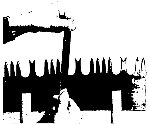
Filing a cutter tooth.
